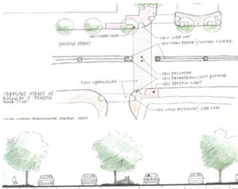
Sketches showing a couple designs for making safer, more attractive roadways and pedestrian crossings
